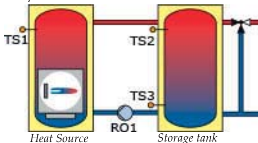
Hydraulic system 3.2
