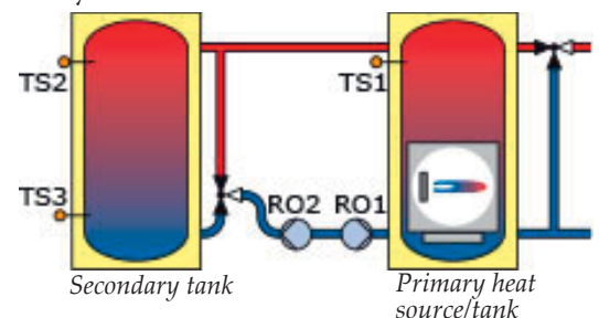
Hydraulic system 1.2
