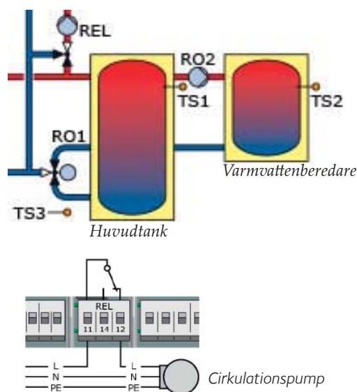
Hydraulschema 4
