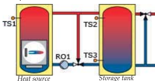
Hydraulic system 3.2
