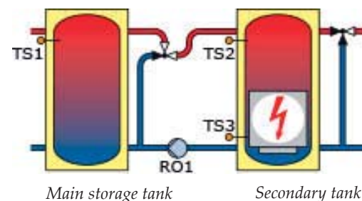
Hydraulic system 2.2
