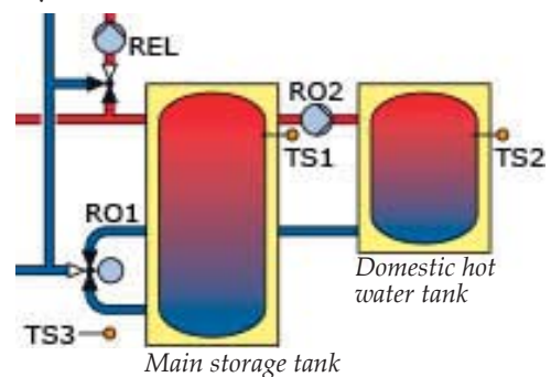
Hydraulic system 4
