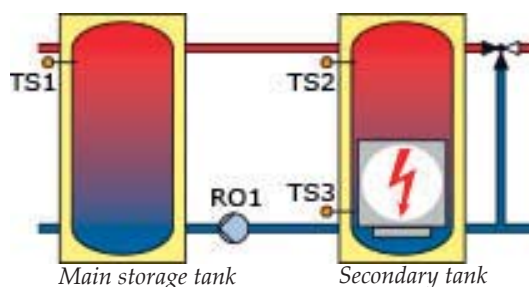
Hydraulic system 2.2
