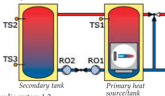
Hydraulic system 1.2
